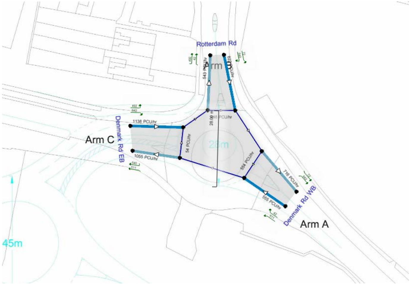
The junction diagram reflects the last run of ARCADY.
